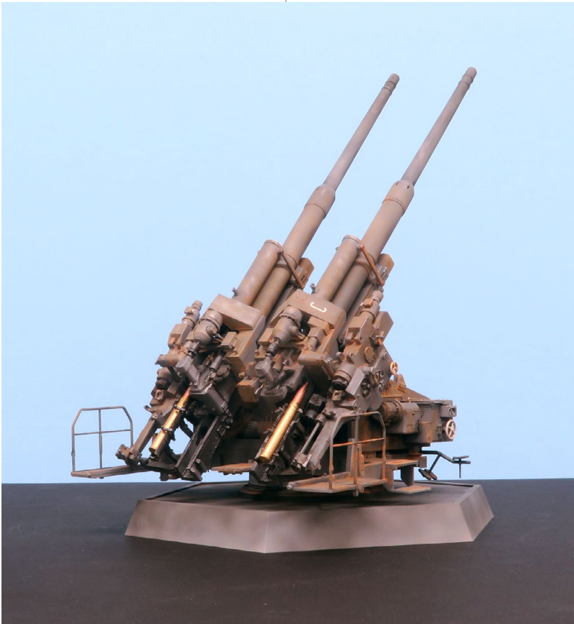
Another shot of Jason Lee's 1:35 scale FlaK 40 Zwilling
